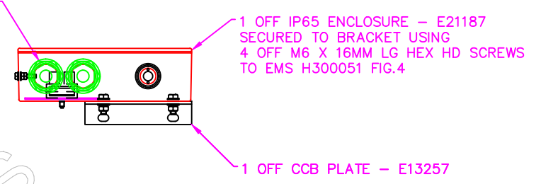
CABLE CHANGE BOX ASSEMBLY.
